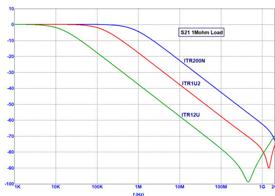
S21 on a 1 M \Omega load
